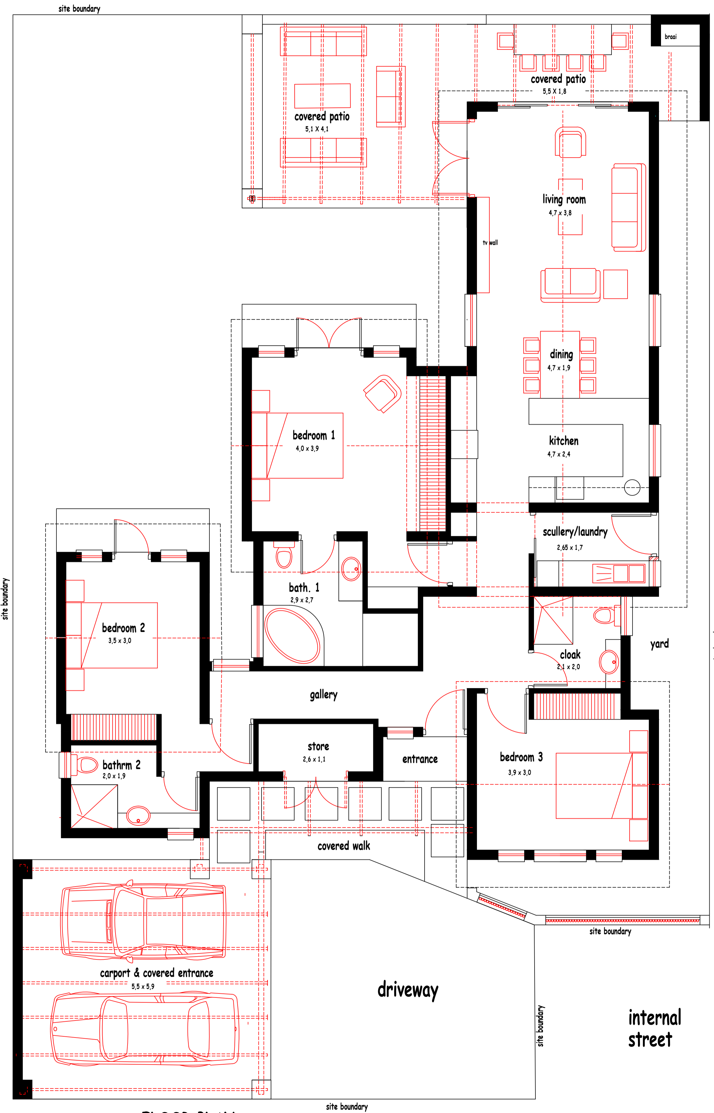
FLOOR PLAN (SOUTH ENTRY)
